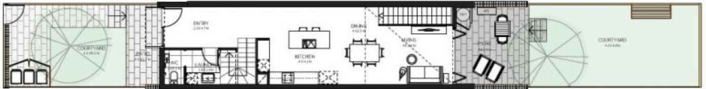
GROUND FLOOR
